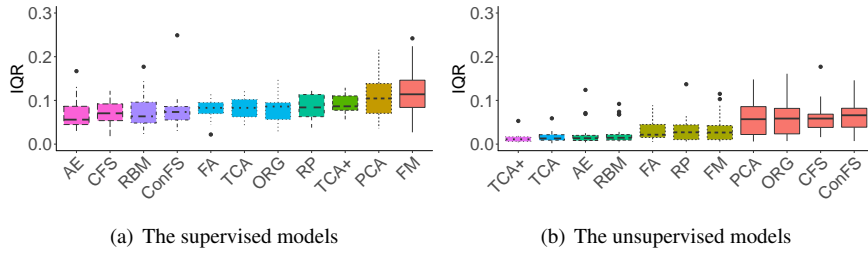
Fig. 9 The Scott-Knott ESD test results for IQR in the supervised and unsupervised models. Each color indicates a rank: feature reduction/selection techniques in different ranks have a significant difference in variance (IQR). Each boxplot has 26 IQR values (one for each project). The x-axis refers to the feature reduction/selection techniques; the y-axis refers to the IQR values.
